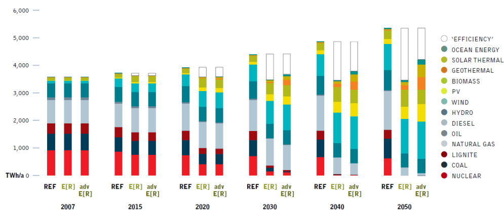
figure 6.36: oecd europe: development of electricity generation structure under 3 scenarios
