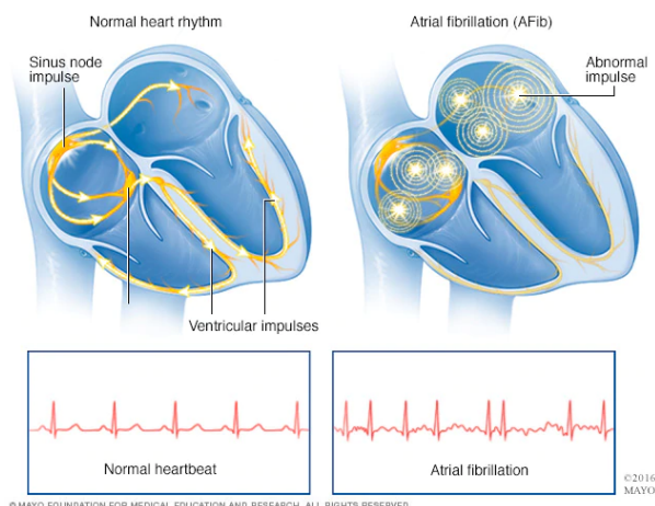
Figure 4: Atrial Fibrillation.
